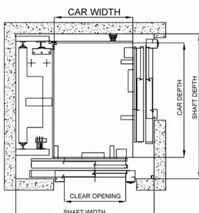
CAR SECTION SIDE OPENING DOORS 2 ENTRANCES FOR ADJACENT OPENING
