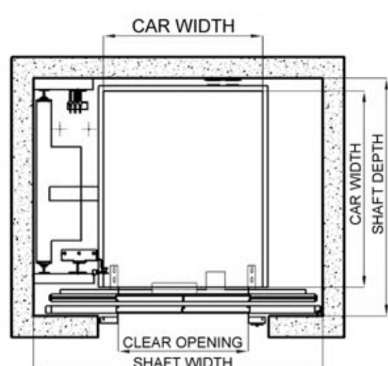
CAR SECTION CENTRE OPENING DOORS SINGLE ENTRY DOORS
