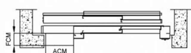
CAR SECTION SIDE OPENING DOORS 2 ACCESSES TO 90°
