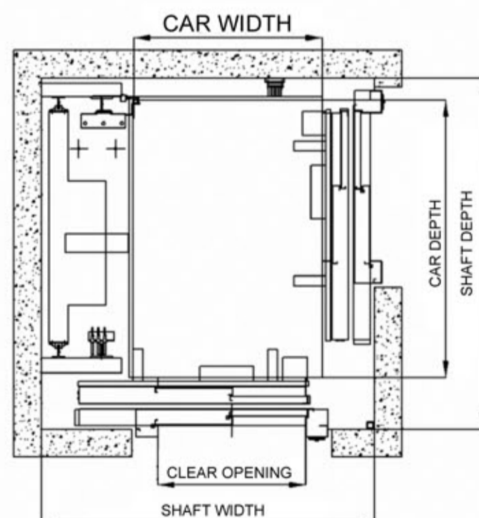
CAR SECTION SIDE OPENING DOORS 2 ACCESSES TO 90°
